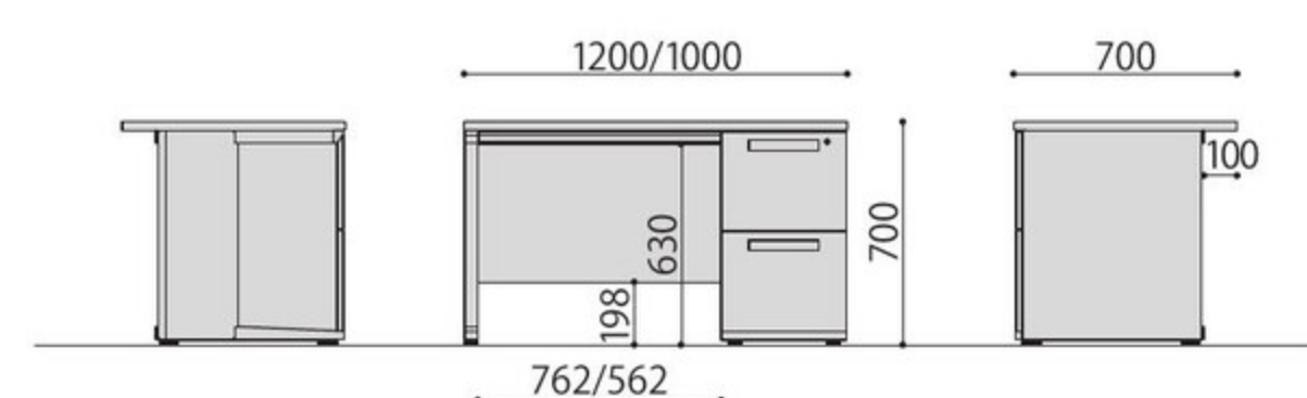
LDC-K107-R2・K127-R2
