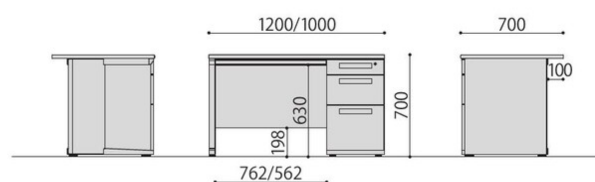
LDC-K107-R3・K127-R3
